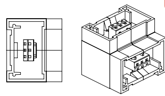
CONECTOR 90° VERTICAL
